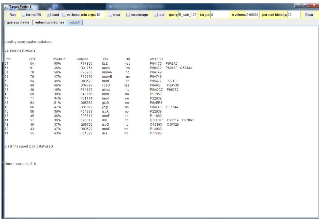
Figure 14: Target Finder: uses BLAST for pairwise sequence alignment and MUSCLE for multiple sequence alignment.
