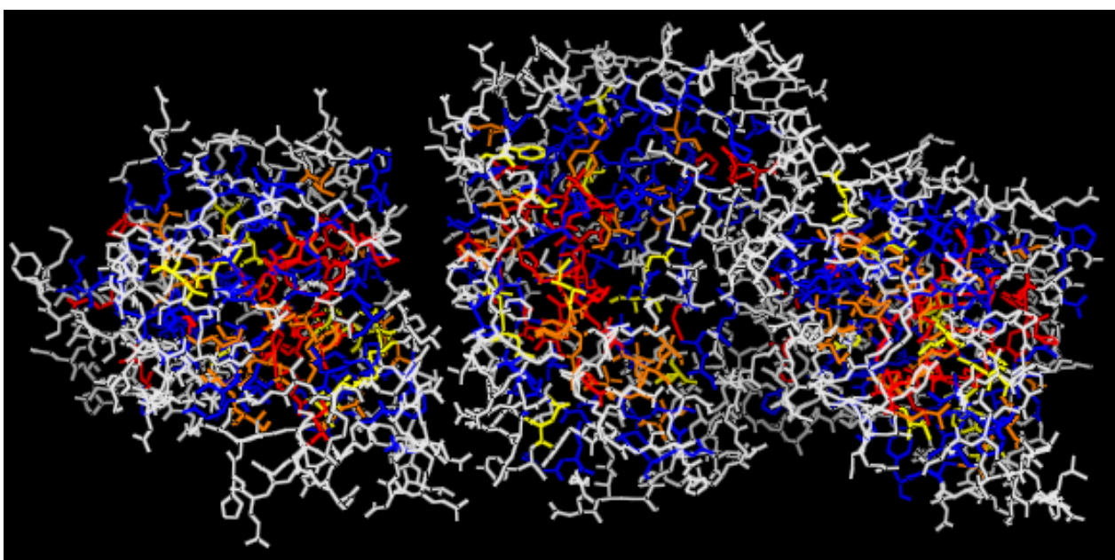
Figure 16: RacE rendered as lines and colored by conservation score: gray {0..5}, blue {6,7}, yellow {8}, orange {9}, red {10,11}. Red indicates highly conserved residues – most of these are internal and not apparent when this molecule is rendered as surface.
