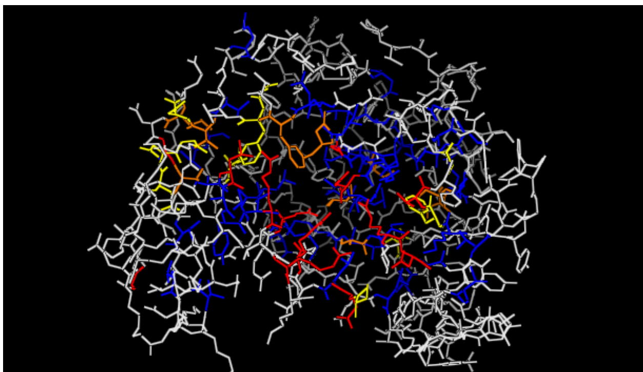
Figure 15: YwtF rendered as lines and colored by conservation score: gray {0.5}, blue {6,7}, yellow {8}, orange {9}, red {10,11}. Red indicates the most highly conserved residues.
