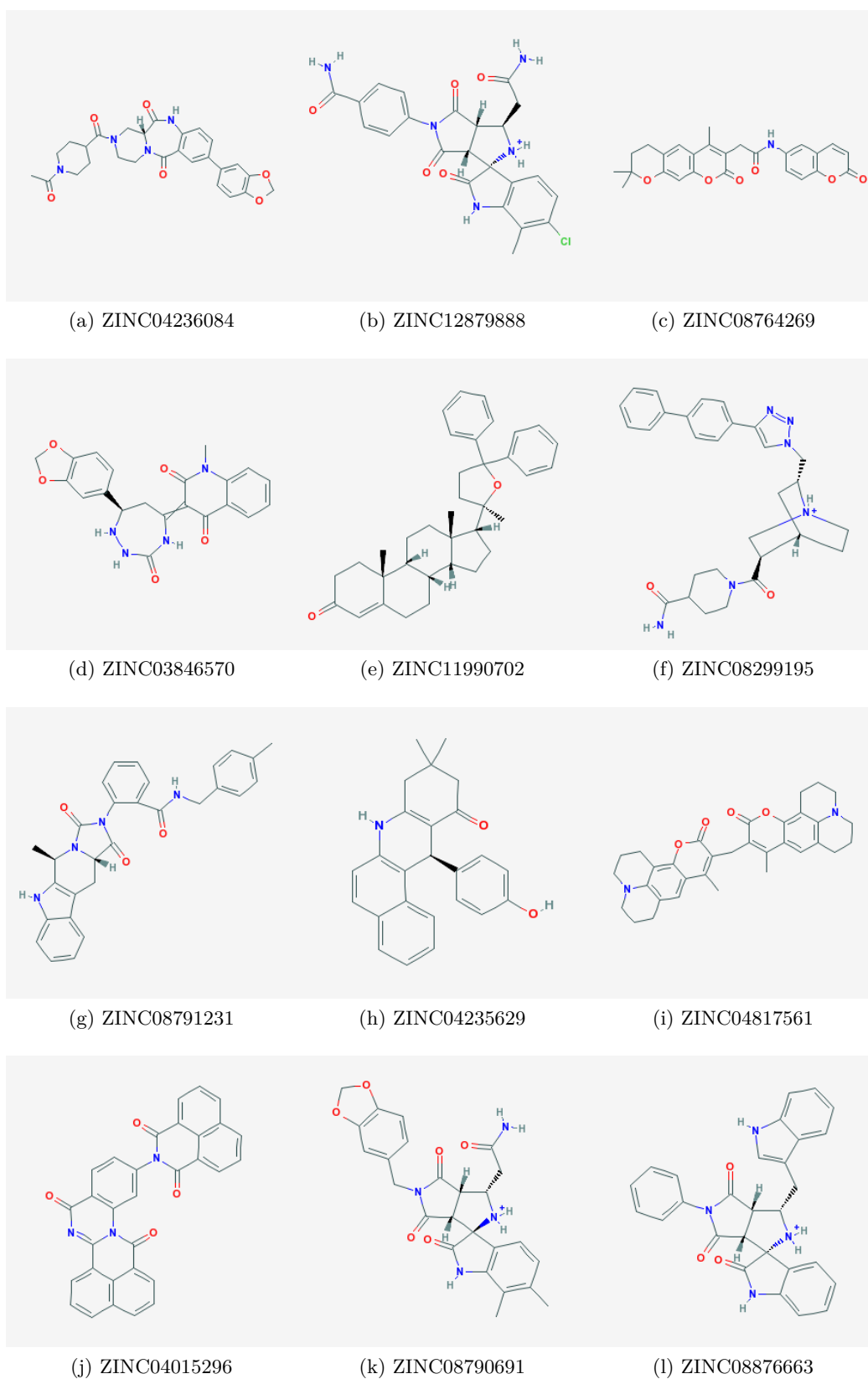
Figure 13: Top scoring ligands for FtsZ (a,b,c) CoaD (d,e,f) YwtF (g,h,i) RacE (j,k,l). Images: http://pubchem.ncbi.nlm.nih.gov .
